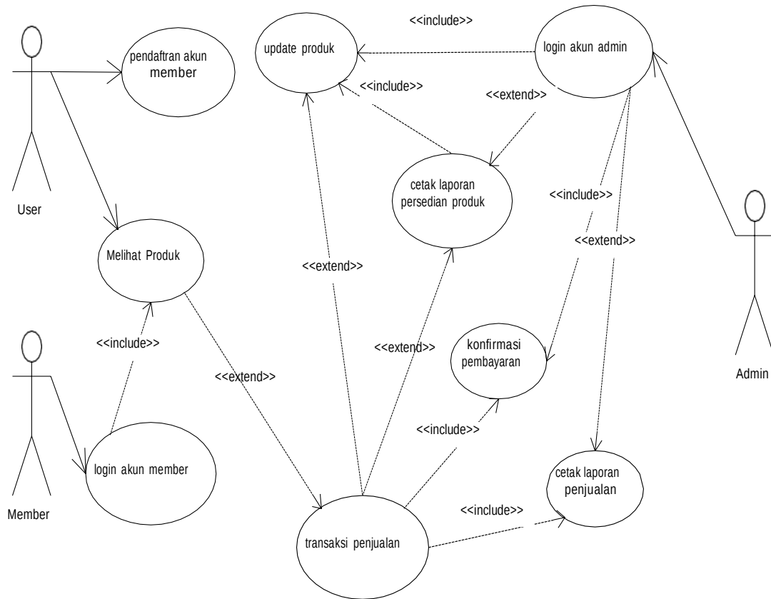
Gambar 3 : Uses Case Diagram
